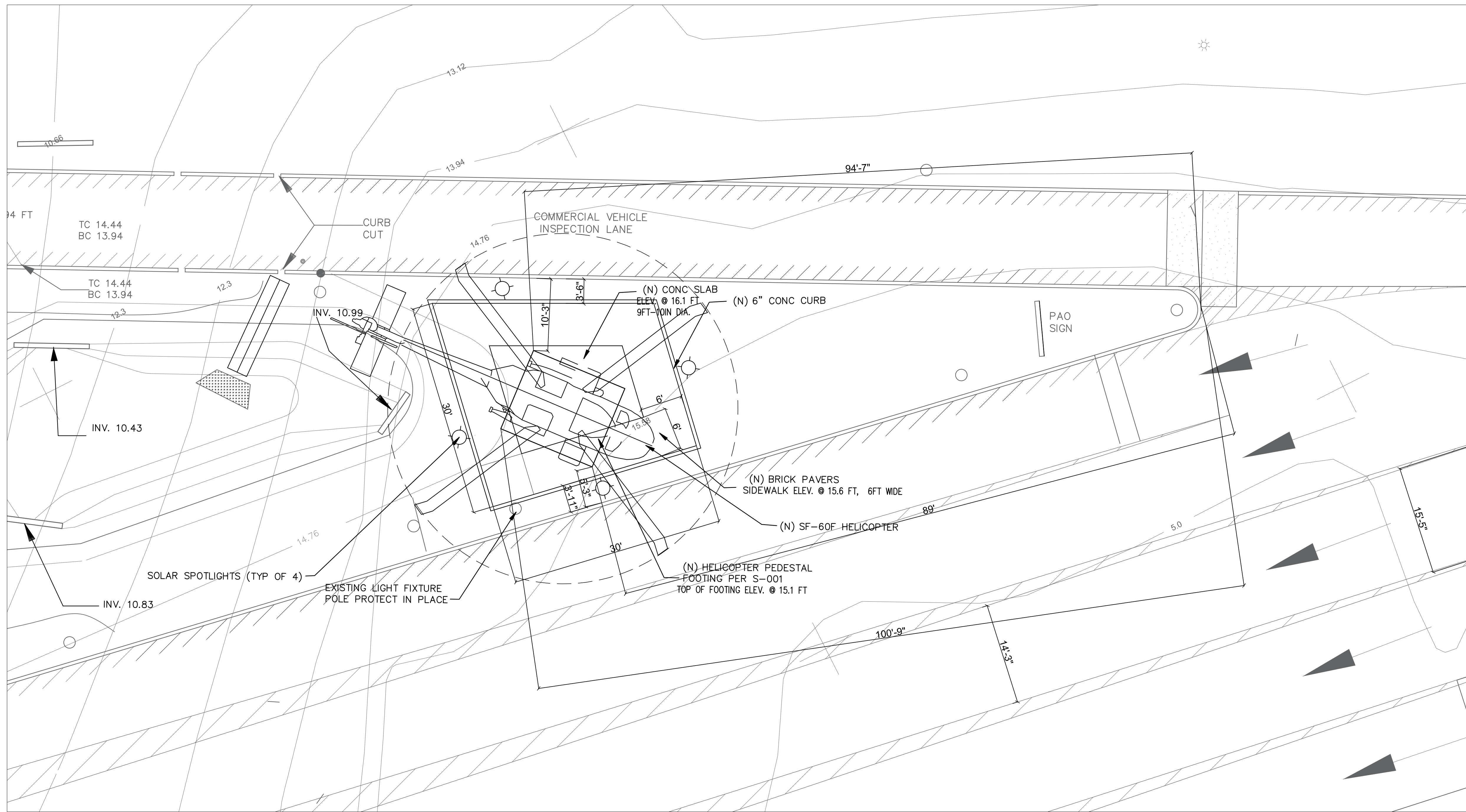
1 ENLARGED SITE PLAN
